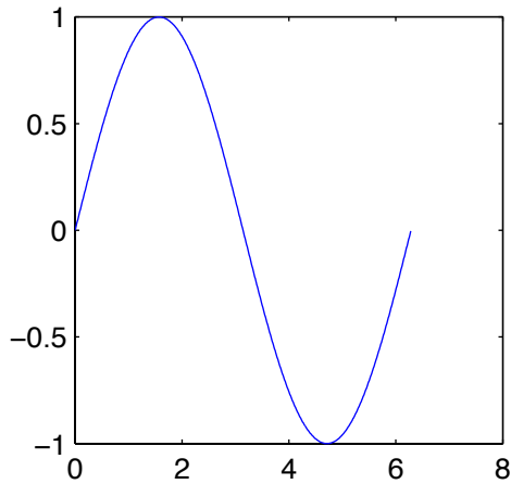
square plot
