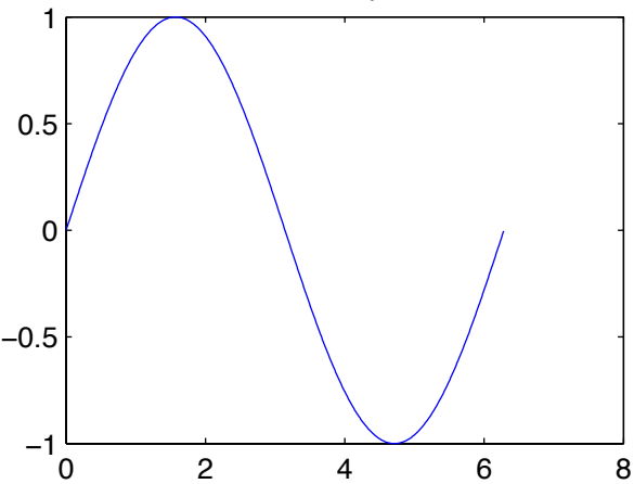
normal plot
