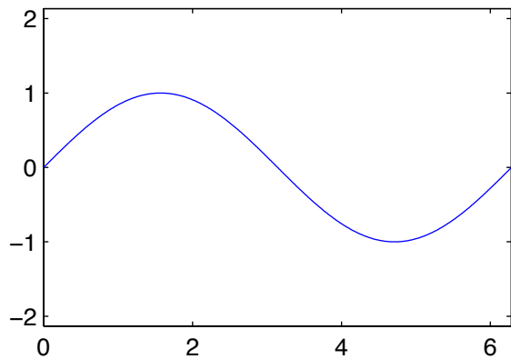
equal plot
